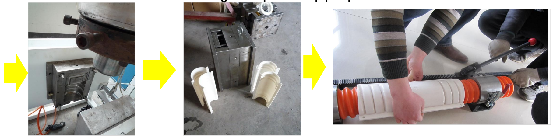
6.Mould clamping machine &Die head mould&Blow moulding
