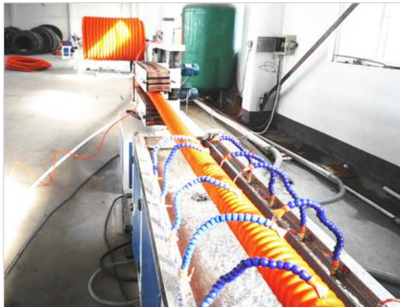
3. Forming machine STCJ-110(Material: stainless steel, inner parts are chromed plated)
